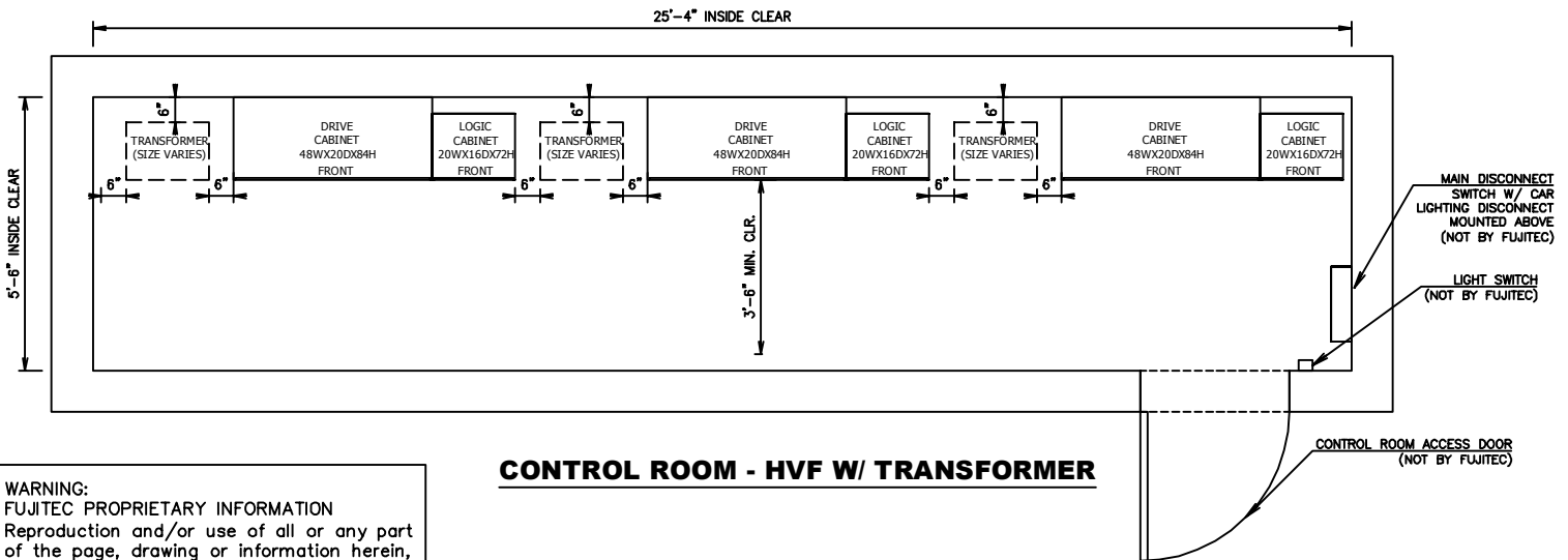
CONTROL ROOM - HVF W/ TRANSFORMER
