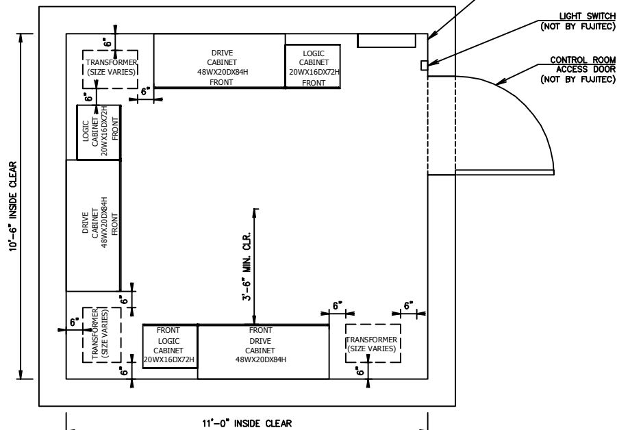
CONTROL ROOM - HVF W/ TRANSFORMER
