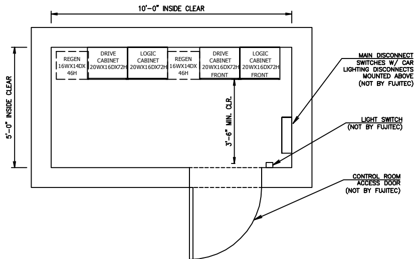
CONTROL ROOM - LVF W/ REGEN
