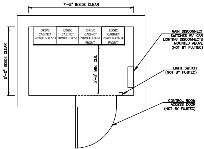
CONTROL ROOM - LVF
