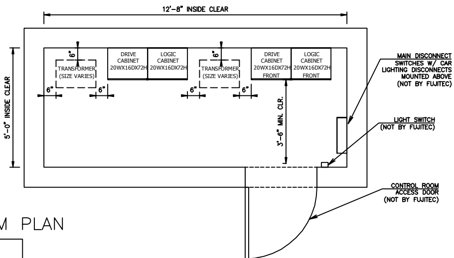
CONTROL ROOM - LVF W/ TRANSFORMER
