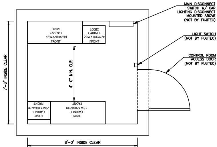
CONTROL ROOM - HVF W/ TRANSFORMER
