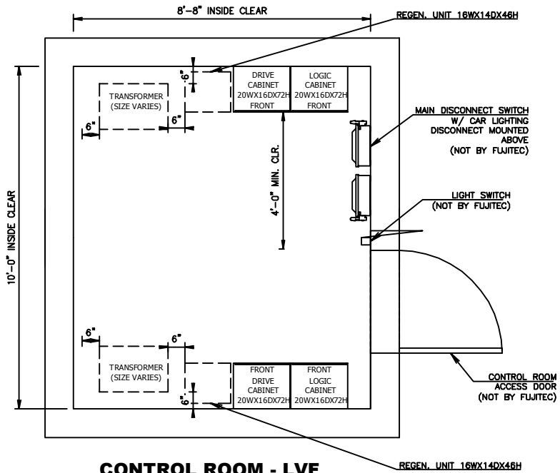
CONTROL ROOM - LVF W/ TRANSFORMER W/ REGEN
