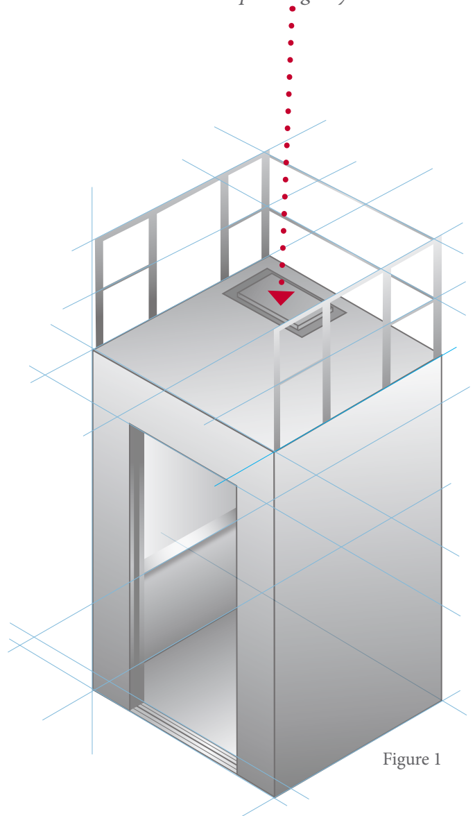
Car Top Emergency Exit
